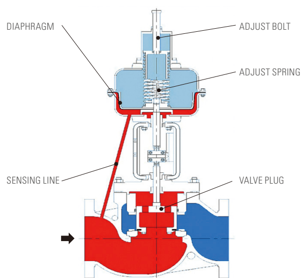
Operational Schematic - Diaphragm Type 2
