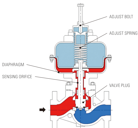
Operational Schematic - Diaphragm Type 1
