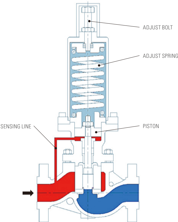
Operational Schematic – Piston Type (Gas)
