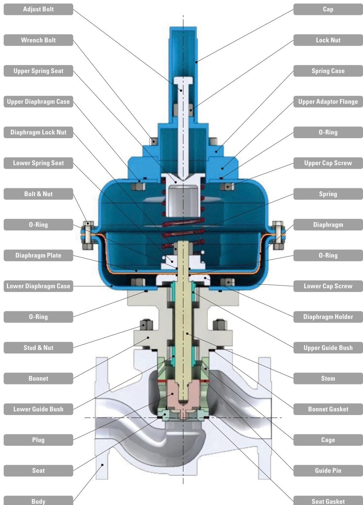
Assembly Drawing (Diaphragm Type)
