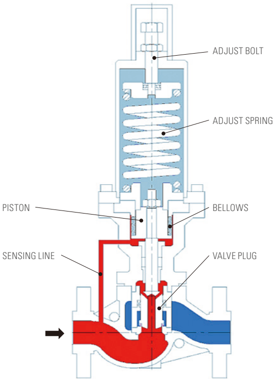
Operational Schematic – Piston Type (Liquid)
