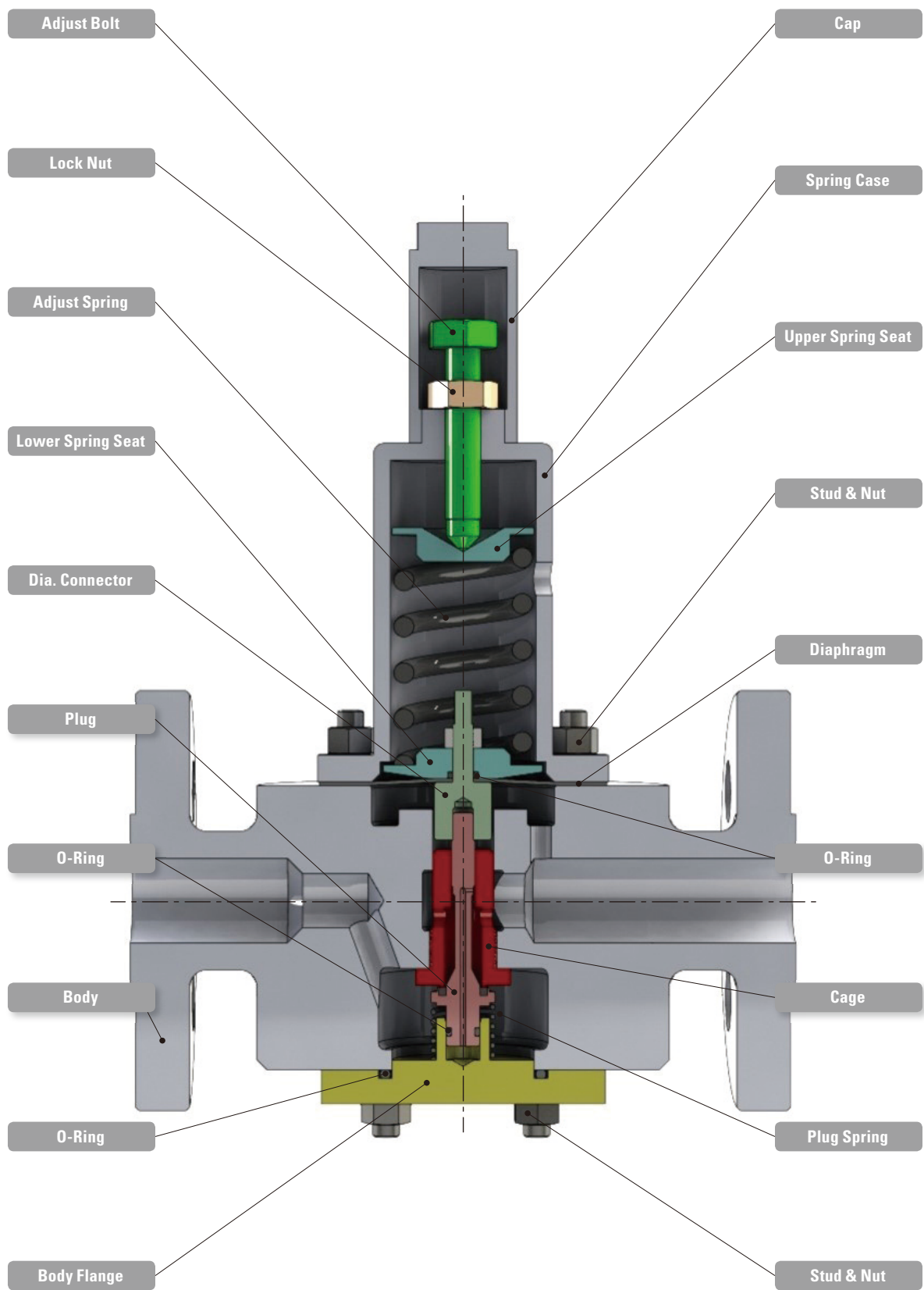
Assembly Drawing (Sectional)
