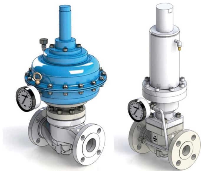
Diaphragm Type
