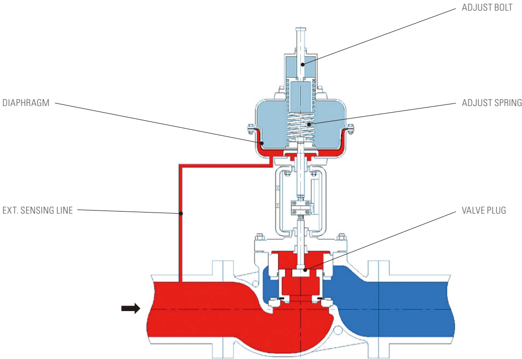
Operational Schematic - Diaphragm Type 3
