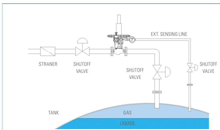
V510 Series Tank Blanketing Valve Installation
